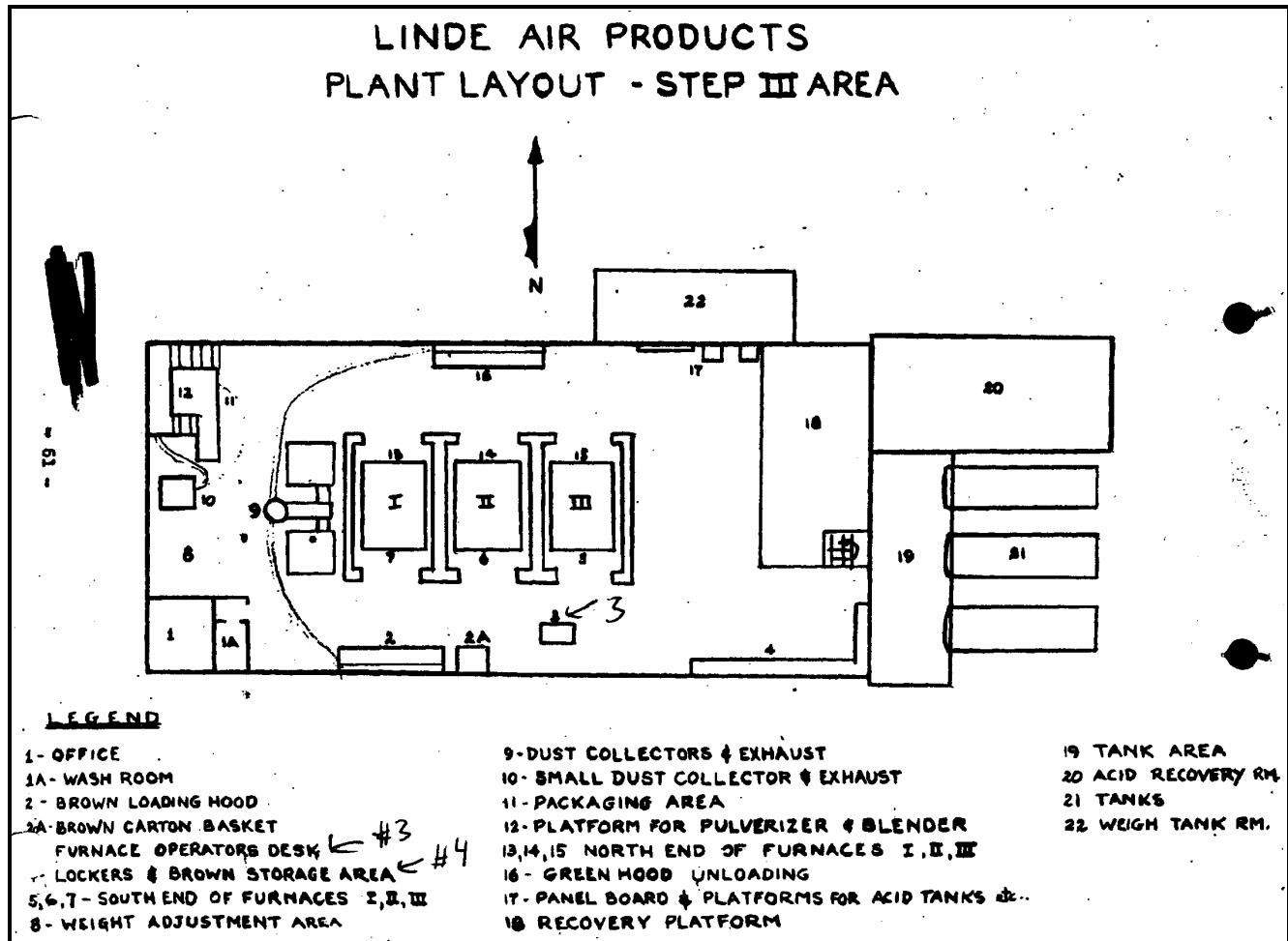
Figure 4. Building 38 layout (from Klewin 1949a).
